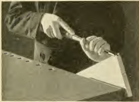
Fig. 8. Chiseling with the Grain.
